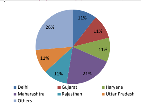
Geographic Diversity (Batch of 2012-14)
