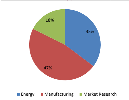
Placement Diversity (Batch of 2011-13)
