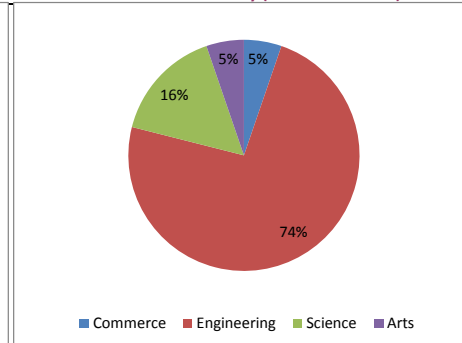
Academic Diversity (Batch of 2012-14)
